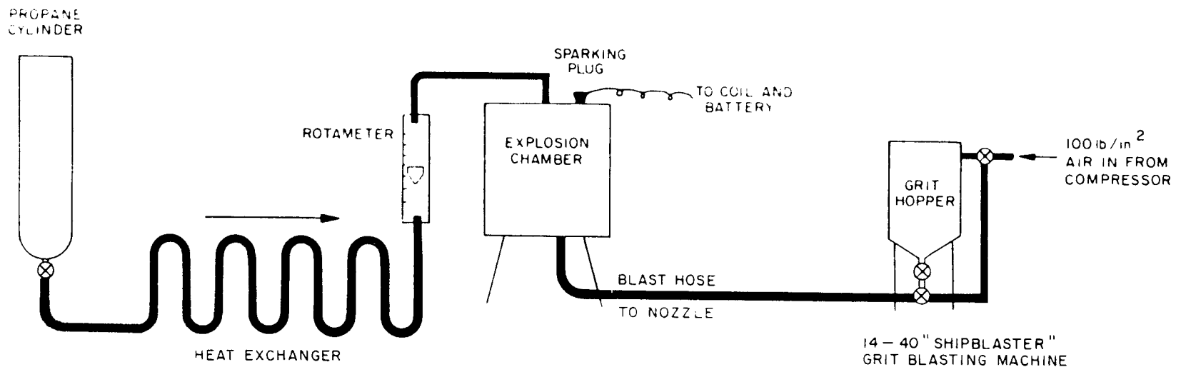
FIG 2 —Diagram of explosion rig
